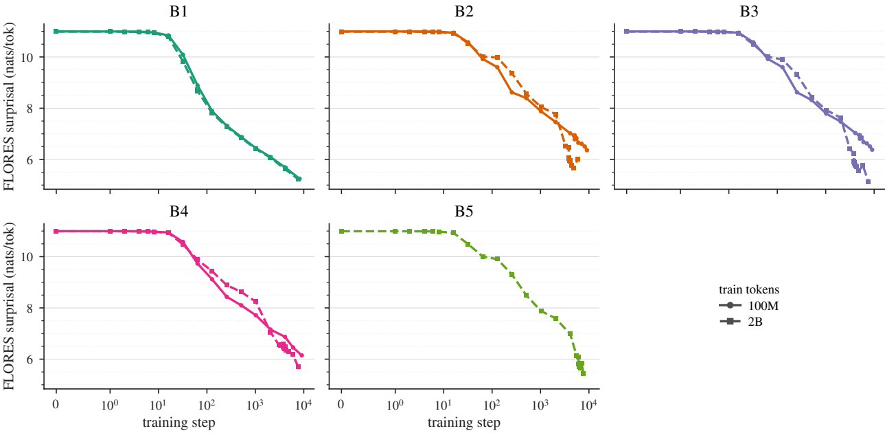
FLORES L2 (English) surprisal across training (mean over nld/deu/zho)
